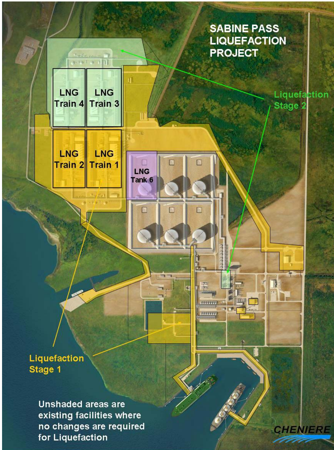
Figure 1.2-2 Liquefaction Stage 1 and Stage 2, Artist Impression – Plan View
